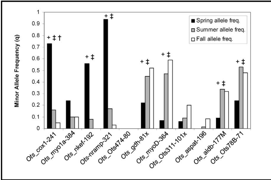
FIGURE 2.—Allele frequencies by Chinook salmon life history types (spring, summer, and fall runs). Validated assays from the screen were tested for their ability to distinguish fish by run timing. Differences in allele frequency were tested for statistical significance by Fisher’s exact test; a single plus sign denotes a significant difference between the spring and summer runs, a double plus sign a significant difference between the spring and fall runs, and a dagger a significant difference between the summer and fall runs.
