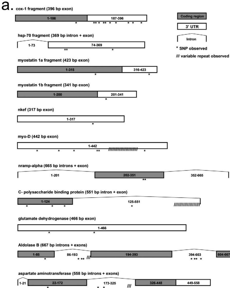
FIGURE 1.—Graphical representation of all sequenced Chinook salmon loci. Panel (a) presents models of each sequenced fragment from a known gene region. The models are broken down into coding, 3' untranslated, and intron regions, and all variations observed in screening are marked. Nonsynonymous single-nucleotide polymorphism (SNP) sites were observed only in the C-polysaccharide binding protein locus. Panel (b) presents models of each sequenced fragment from each microsatellite locus, showing sequenced DNA regions in relation to the repeated sequence. The repeated sequence was not included in the numbering of sequenced base pairs (bp).
